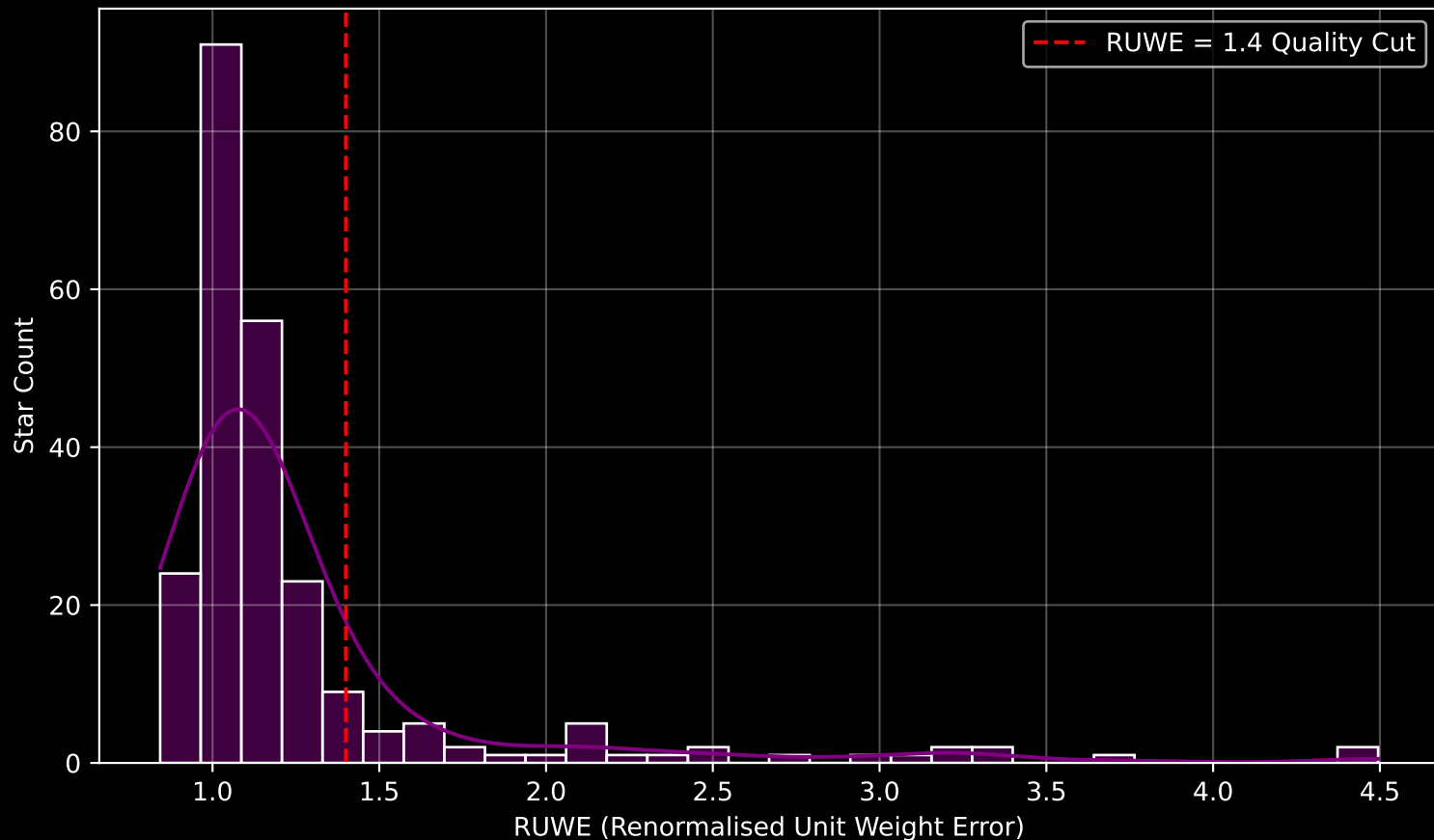
GALAH DR4 Field [8959] RUWE Distribution (n= 235)
