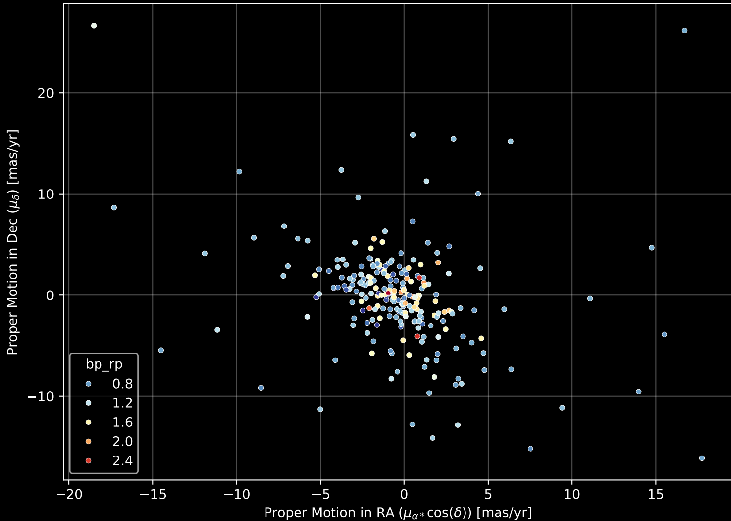
GALAH DR4 Field: [8959] Proper Motion Diagram (n= 242)
