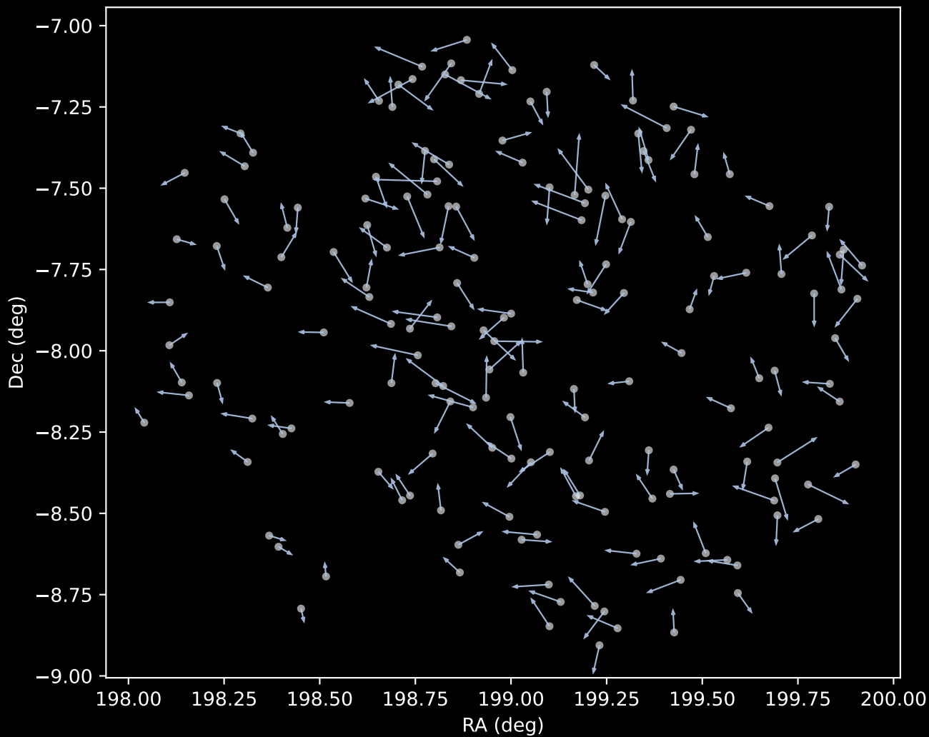
GALAH DR4 Cluster 1 Proper Motion Vectors (n=171)
